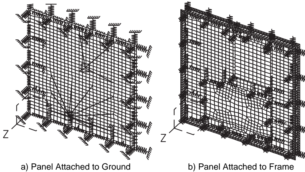
Figure 4: Structural Finite Element Models
