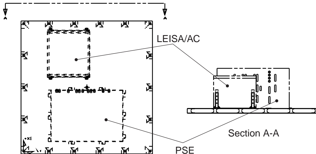
Figure 1: Carbon-Carbon Radiator with Attached Electronics Boxes. (Drawing provided by SAI 1 )
