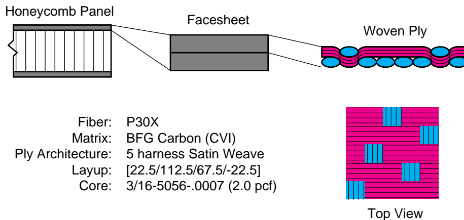
Figure 2: Facesheet Design
