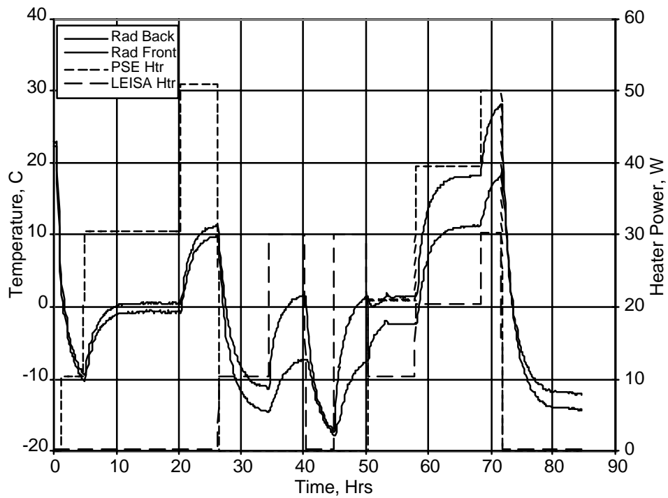
Figure 11: Thermal Balance Test – Radiator Temps & Heater Powers
