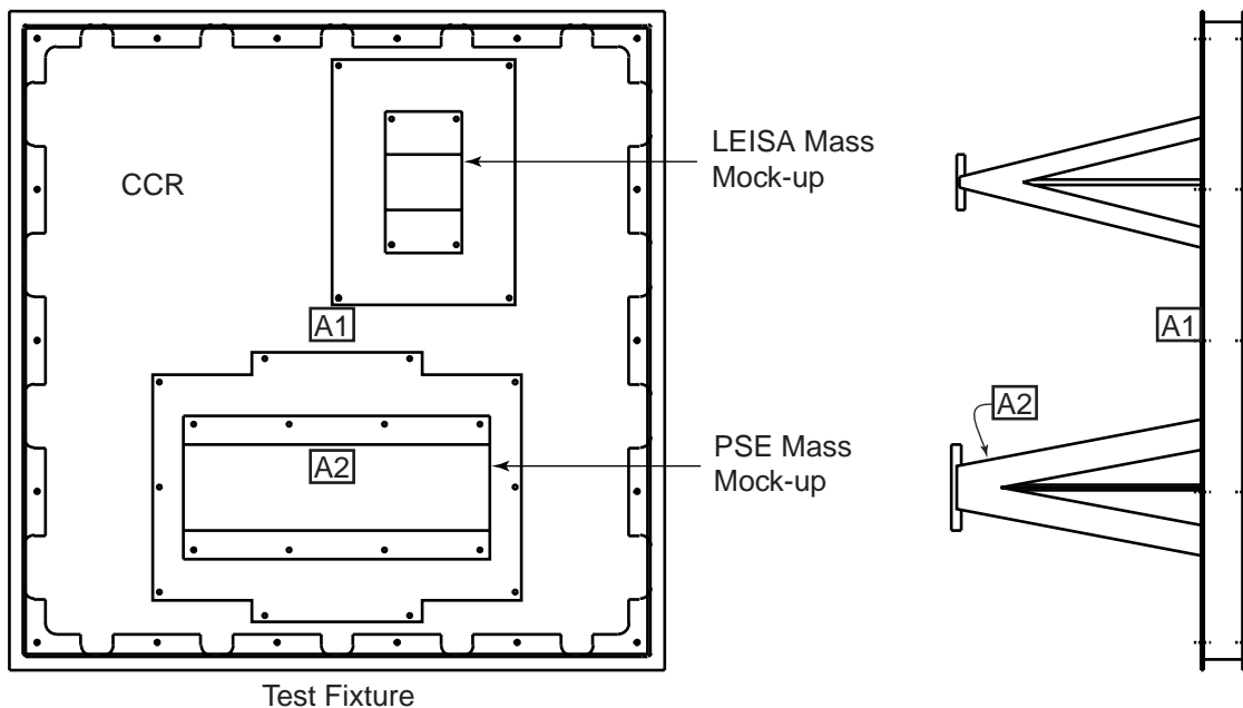
Figure 16: Vibration Test Configuration
