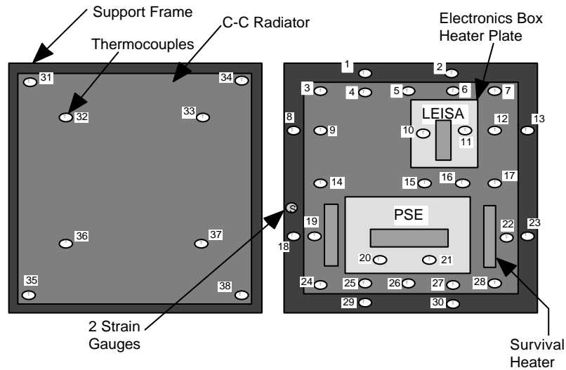
Figure 6: Thermocouple and Strain Gauge Locations for the Carbon-Carbon Radiator Thermal Vacuum Test
