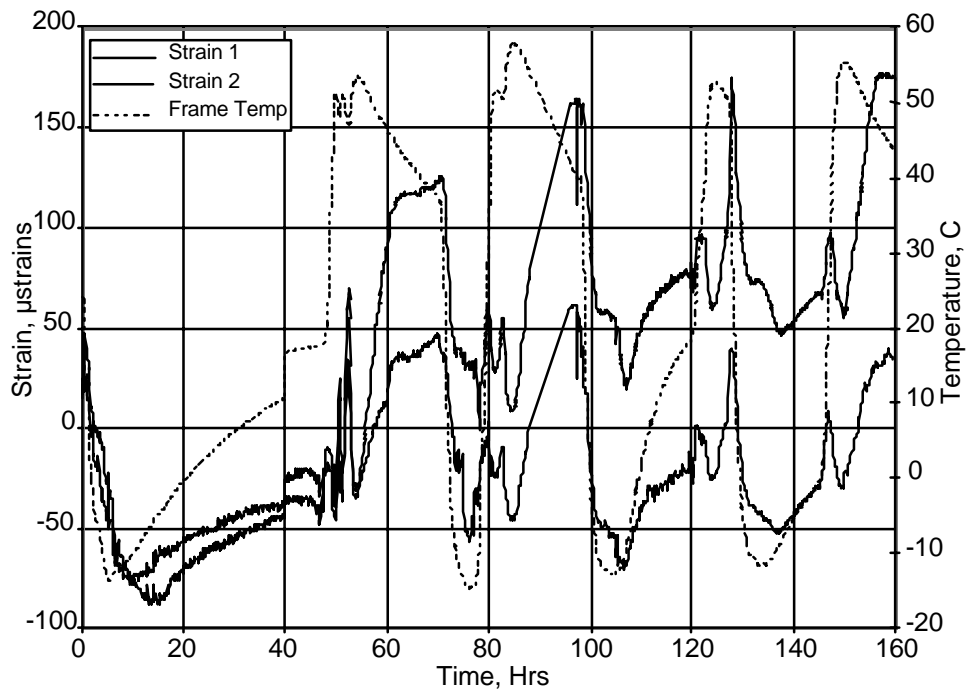
Figure 10: Thermal Cycles Test – Strain Gauges
