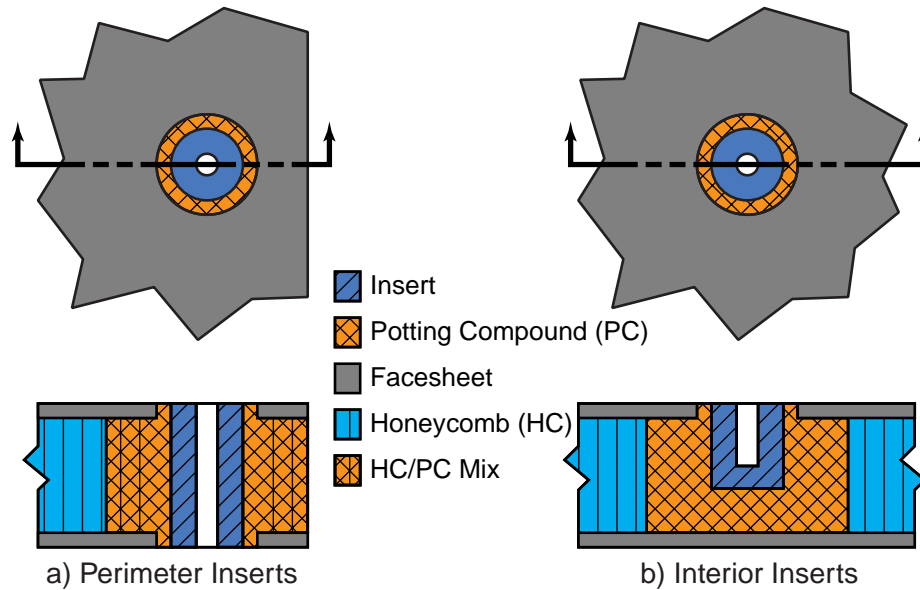
Figure 3: Insert Design
