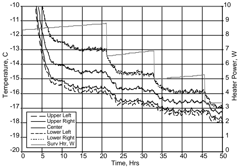
Figure 13: Survival Heater Test – Radiator Back
